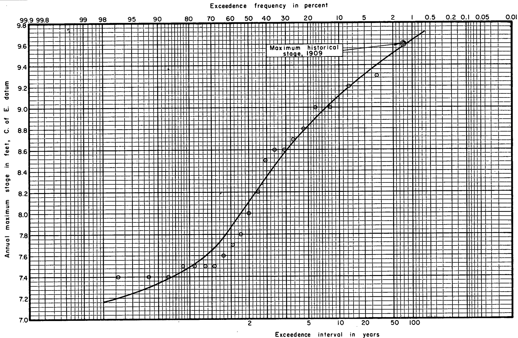
ILLUSTRATIVE EXAMPLE RIVER STAGE FREQUENCY CURVE, 1935-1956
