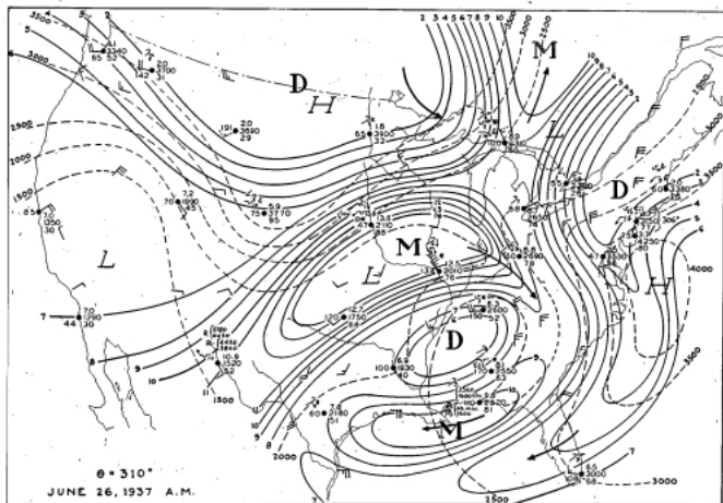
Isentropic Chart for June 26, 1937
