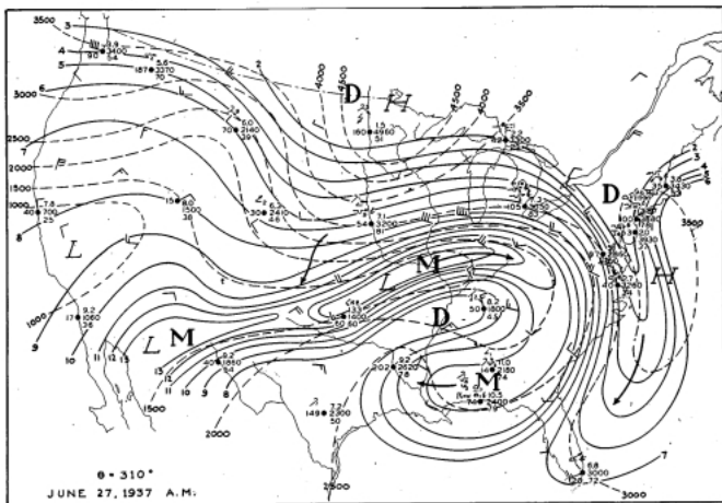
Isentropic Chart for June 27, 1937
