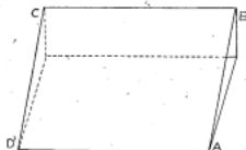
FIG. 14. The sloping isentropic surface.
