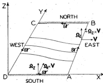
FIG. 3. The direction of the vertical component \Omega_z of the earth's angular velocity and of the cross product \Omega_z \times \mathbf{v} within the wave.
