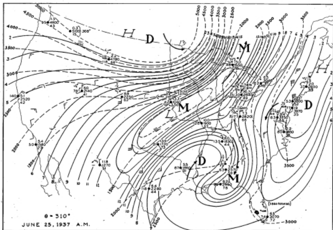
Isentropic Chart for June 25, 1937. Solid lines are lines of specific humidity while dotted lines are lines of elevation (in meters) of the chosen surface above sea level. "M" signifies the center of a moist tongue, "D" the center of a dry tongue. "H" and "L" are entered at the crests and troughs of the isentropic sheet. The numbers to the right of the aerological stations are, in the order listed, the specific humidity, the elevation, and the relative humidity at the given isentropic sheet.
