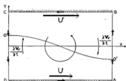
Fig. 8. The action of the local accelerations \partial v_x/\partial t in causing the amplitude of the wave to increase (instability).
