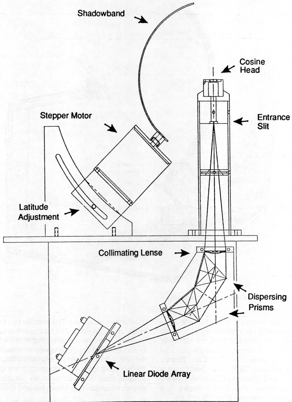
Figure 23. The Rotating Shadowband Spectrometer.
