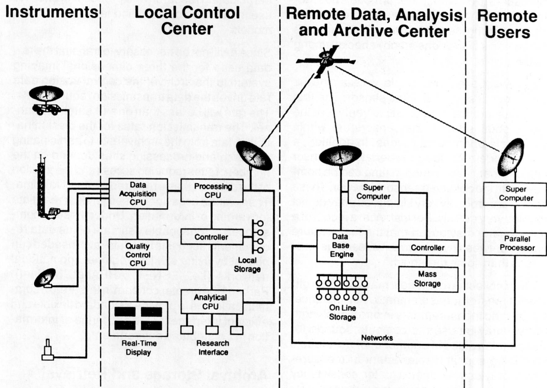
Figure 18. Components of the ARM data management system.
