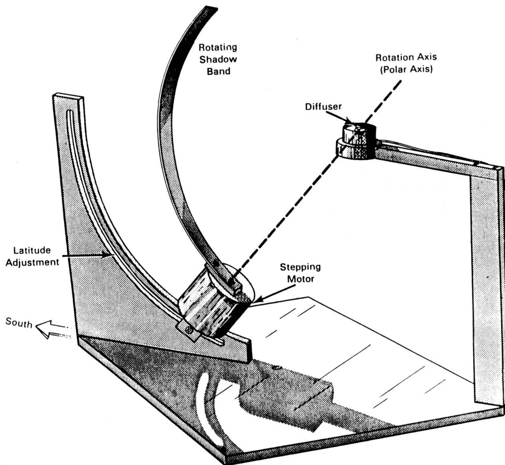
Figure 22. The Rotating Shadowband Radiometer.
