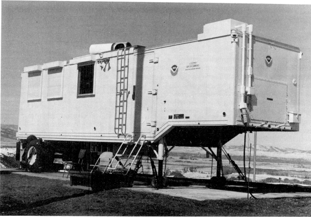
Figure 14. The NOAA mobile lidar unit.
