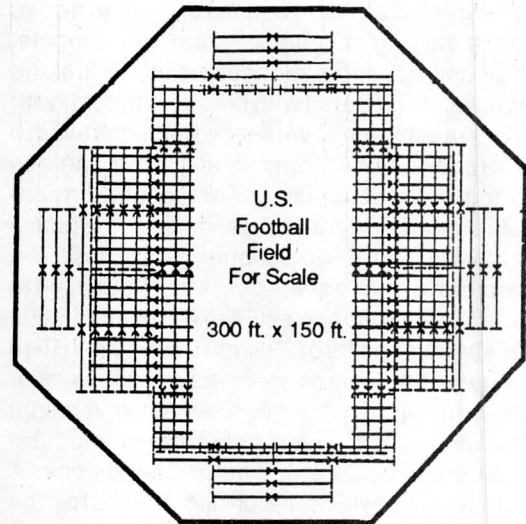
Figure 24. A large-scale RASS antenna array.
