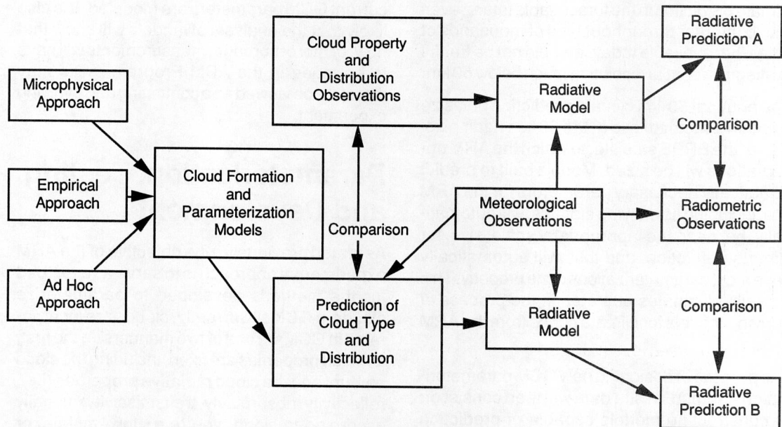
Figure 8. Linkages of the cloud parameterization, radiation modeling and observation programs. The critical activity of the various comparisons is hypothesis testing. Although not shown, the results of the comparisons feedback to the various modeling programs.
