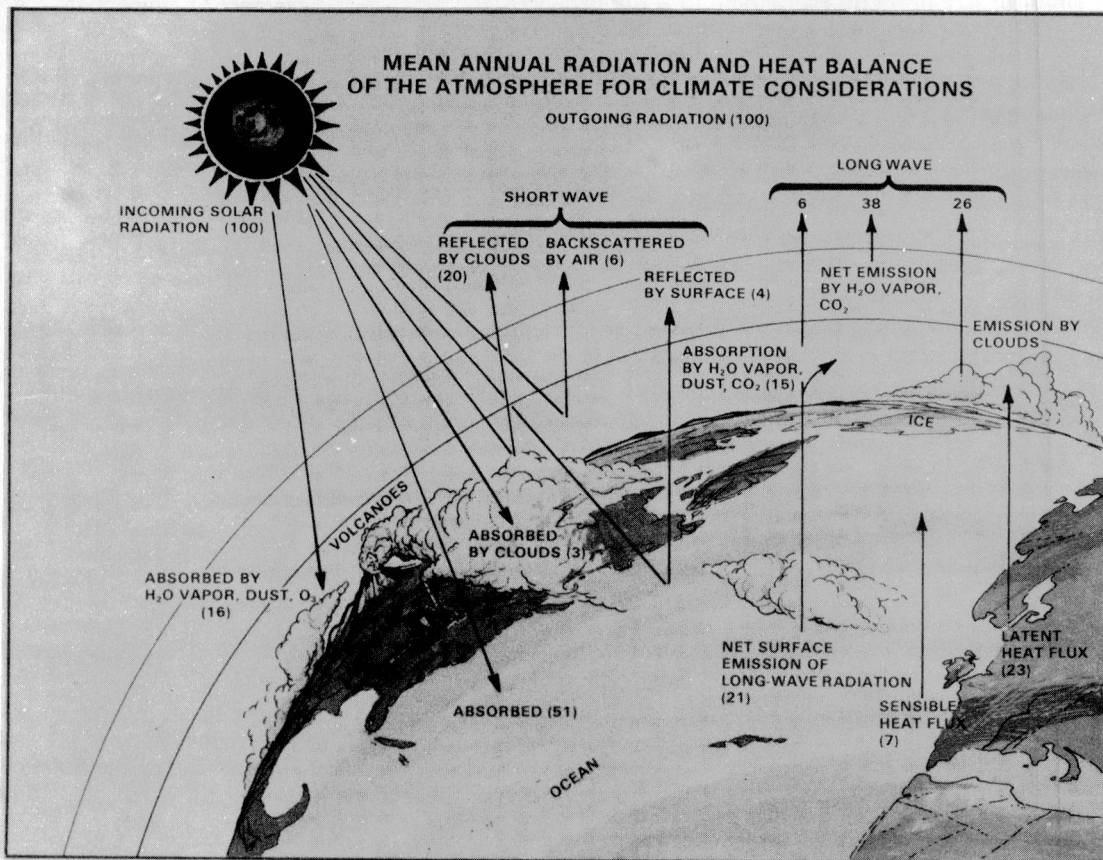
Figure 1. Mean annual radiation and heat balance of the atmosphere for climate considerations.
