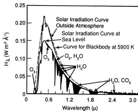
Figure 4. Spectral distribution curves related to the sun. The shaded areas indicate absorption, at sea level, due to the atmospheric constituents shown. (From Gast et al.; McGraw-Hill 1965.)
