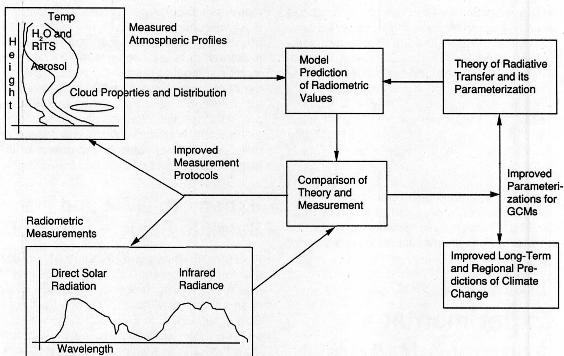
Figure 7. The ARM experimental approach as applied to the study of the radiation field.
