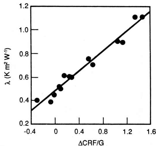
Figure 5. Cess intercomparison findings: model sensitivity vs. cloud radiative forcing.
