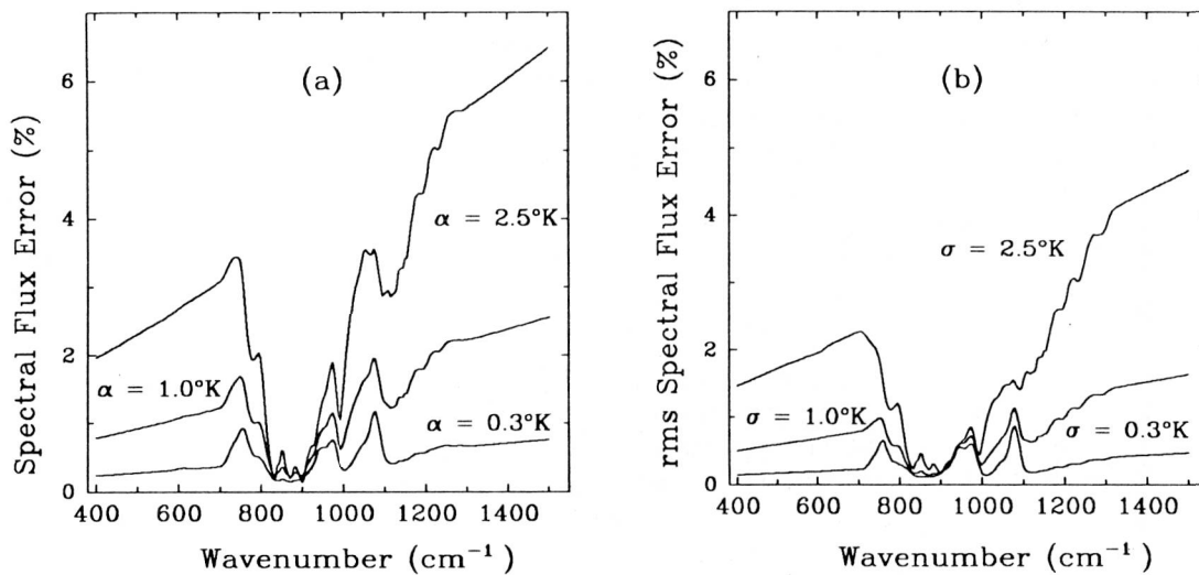
Figure 10. As in Figure 9 but for the temperature distribution. The perturbations ( \alpha ) and standard deviations ( \sigma ) are given in Kelvins.
