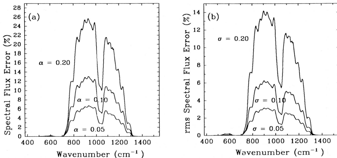
Figure 9. Spectral distribution of possible errors in calculated spectral flux (or intensity) due to systematic (a) and random (b) errors in the tropospheric water vapor distribution. Calculations were performed with LOWTRAN7 for the AFGL midlatitude summer atmosphere. Fractional systematic perturbations are denoted by \alpha , and \sigma is the standard deviation of the assumed normally distributed error. The calculations were done every 5\text{ cm}^{-1} , although the LOWTRAN7 transmittances are averages over 20\text{ cm}^{-1} .
