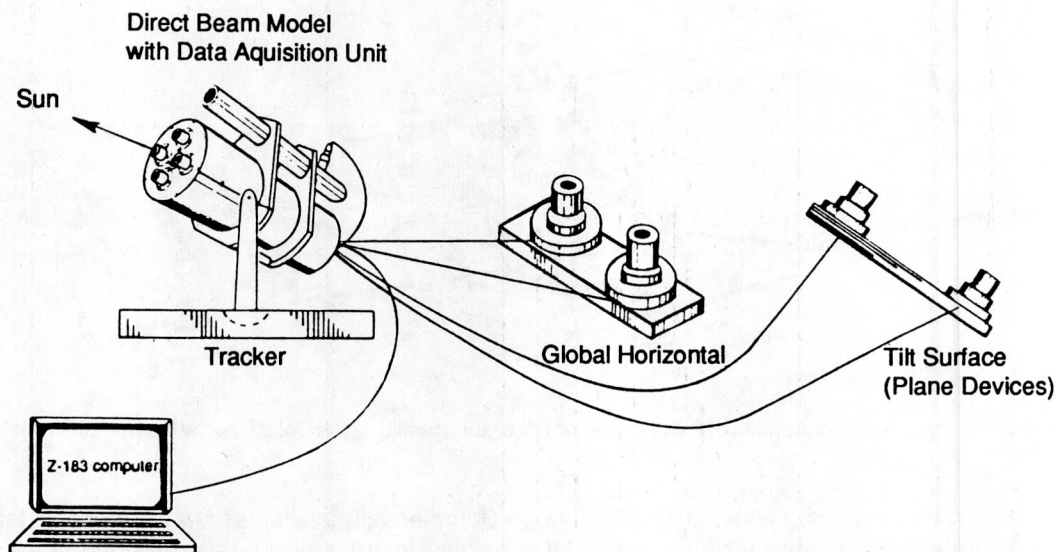
Figure 16. The calibration of radiometric instruments often involves the intercomparison of different kinds of sensors using the sun as the calibration source. A fairly common method of calibration involves the use of a tracking radiometer. The system shown here is in use at SERI.
