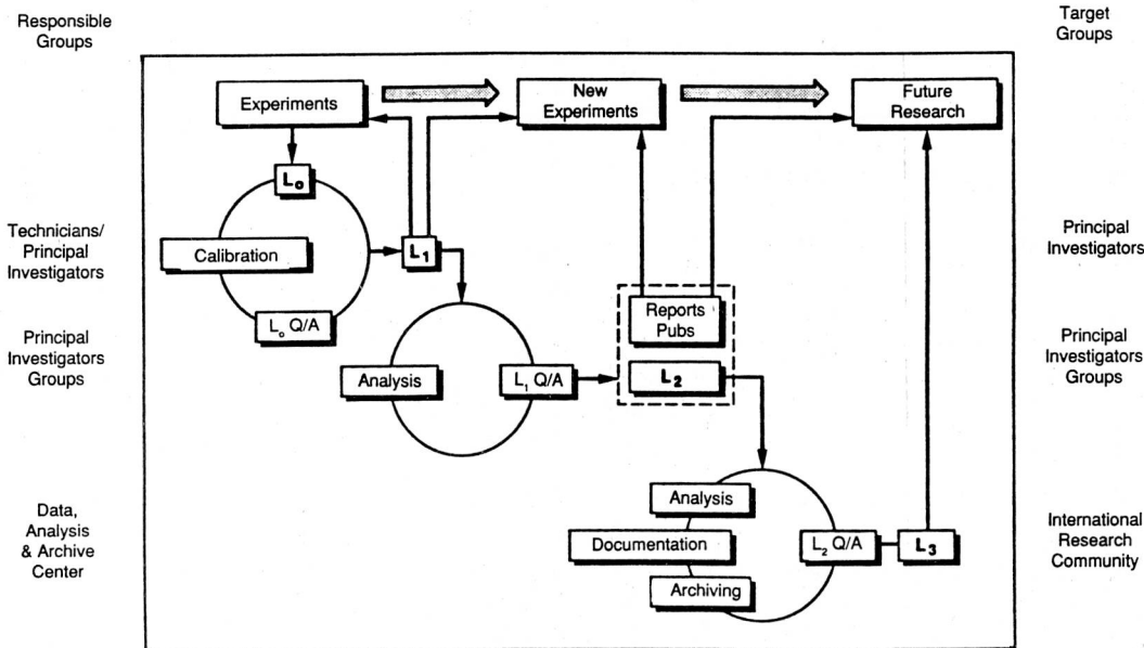
Figure 17. Conceptual design of ARM data flow.
