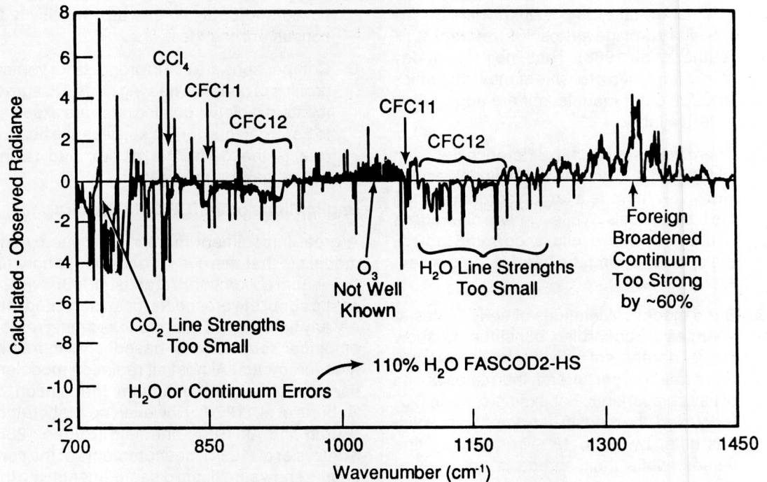
Figure 6. The difference between FASCOD2-calculated and HIS-measured radiance spectra found by Dr. William Smith, University of Wisconsin.
