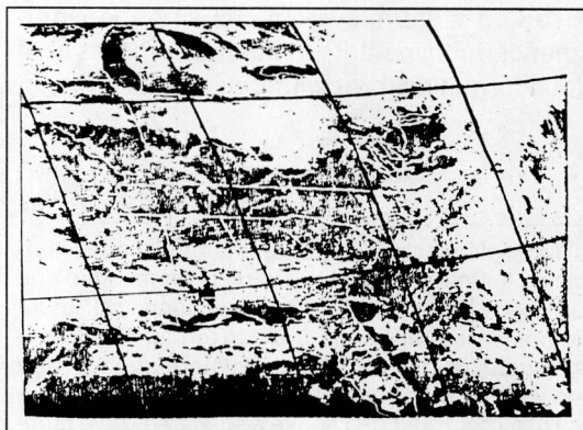
Figure 3. The GCM grid of Figure 2 superimposed on a storm system in the Southeast U.S.
