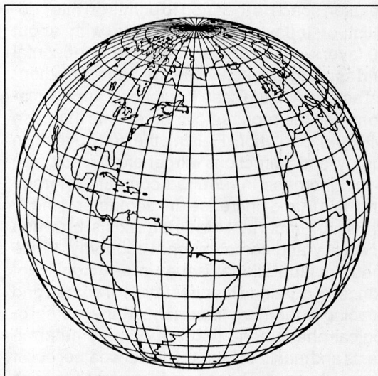
Figure 2. A typical GCM global grid scale.
