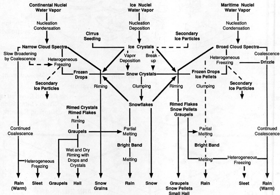
Figure 13. An idealized representation of the generation and metamorphosis of cloud and precipitation particles.
